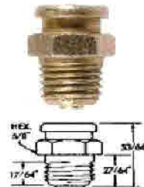
1/4" NPT Pipe Thread Standard Button Head Fitting Part No. 83-B-412
