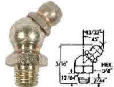
1/4"-28 Pipe Thread 45° Angle Part No. 83-F-445
