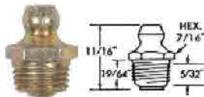
1/8" N.P.T. Pipe Thread Straight Part No. 83-212
