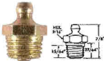
1/4" Pipe Thread Straight / Up to 10,000 PSI Part No. 83-414
