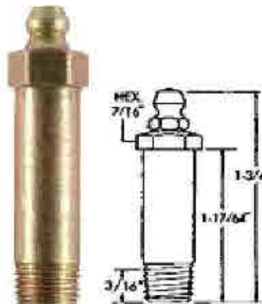
1/8" N.P.T. Pipe Thread Straight (1-3/4" Length) Part No. 83-228L
