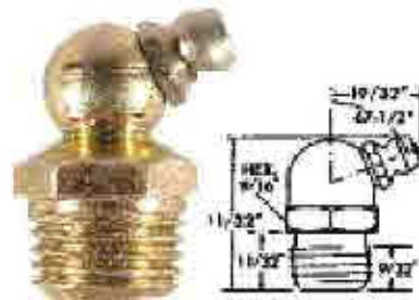
1/4" Pipe Thread 67-112° Angle / Up to 10,000 PSI Part No. 83-468
