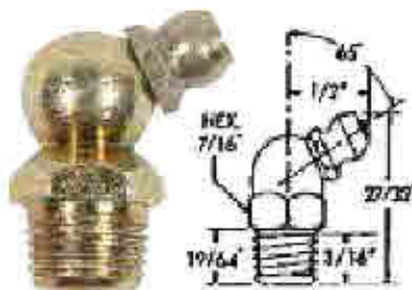
1/8" N.P.T. Pipe Thread 65° Angle Part No. 83-268
