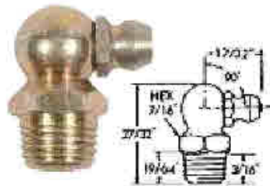
1/8" N.P.T. Pipe Thread 90° Angle Part No. 83-290
