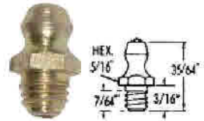
1/4"-28 Pipe Thread Straight Part No. 83-F-410
