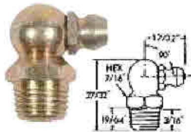
1/8" N.P.T. Pipe Thread 90° Angle Part No. 83-290
