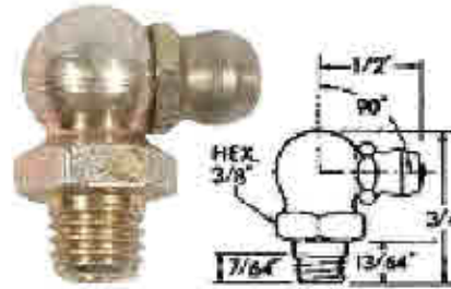
1/4"-28 Pipe Thread 90° Angle Part No. 83-F-490
