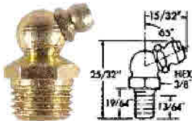
1/4"-28 Pipe Thread 65° Angle Part No. 83-F-468
