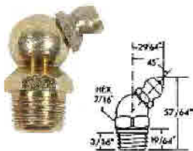
1/8" N.P.T. Pipe Thread 45° Angle Part No. 83-245
