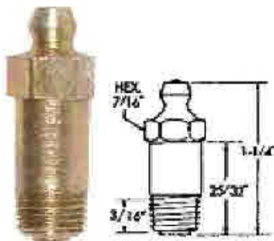
1/8" N.P.T. Pipe Thread Straight (1-1/4" Length) Part No. 83-228
